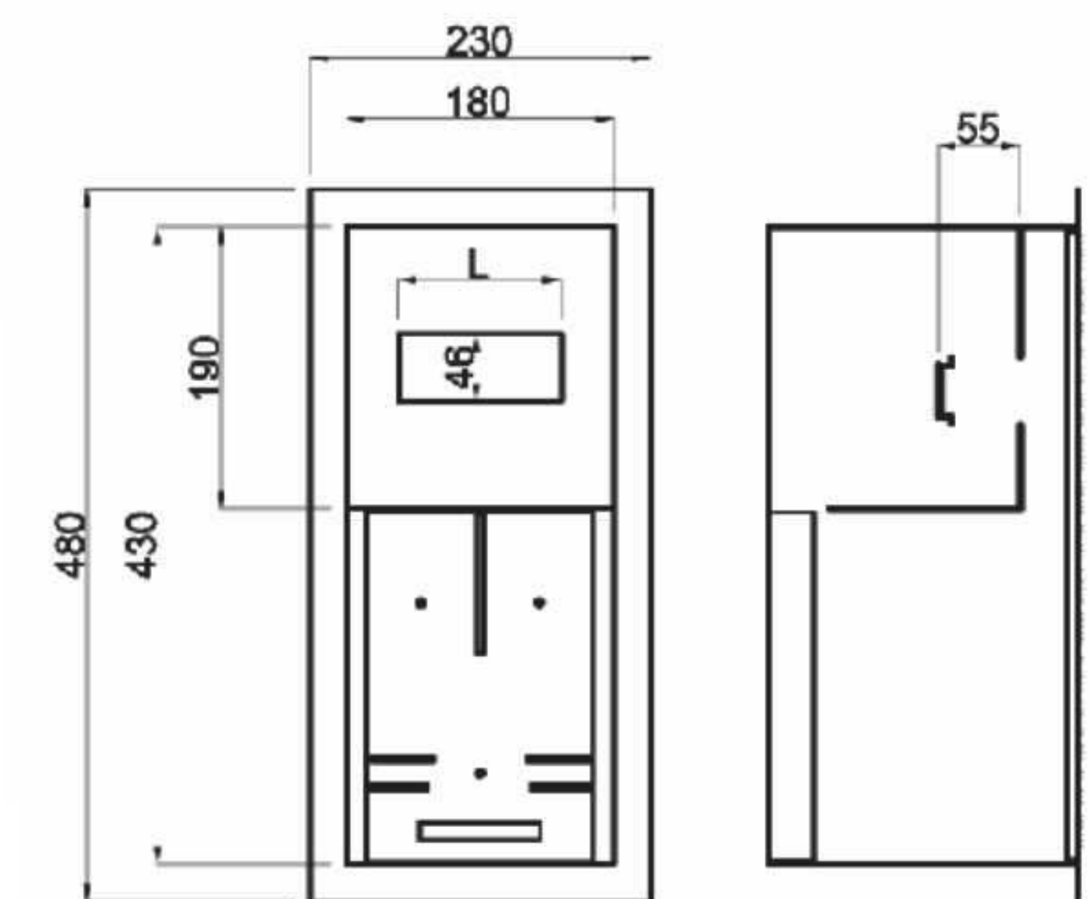
RLP-1F-1 L=18 RLP-1F-3 L=55 RLP-1F-6 L=110 RLP-1F-12L=220
